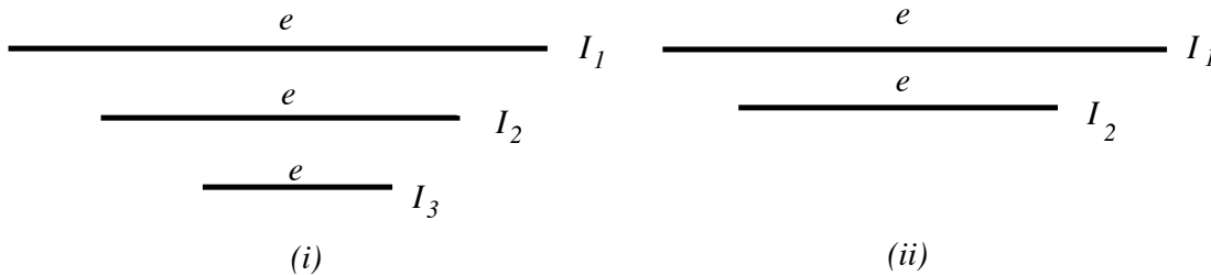
Fig. 1. Two models making \phi true at any I \supseteq I_1 .
