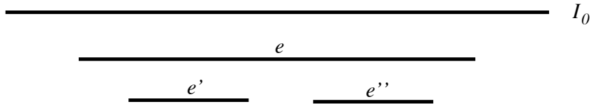
Fig. 4. A model for \varphi .
