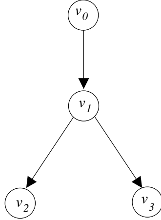
Fig. 3. The graph after the existential node expansion rule expands \psi' and \psi'' .
